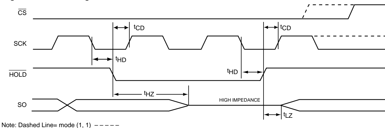
Figure 9. HOLD Timing
