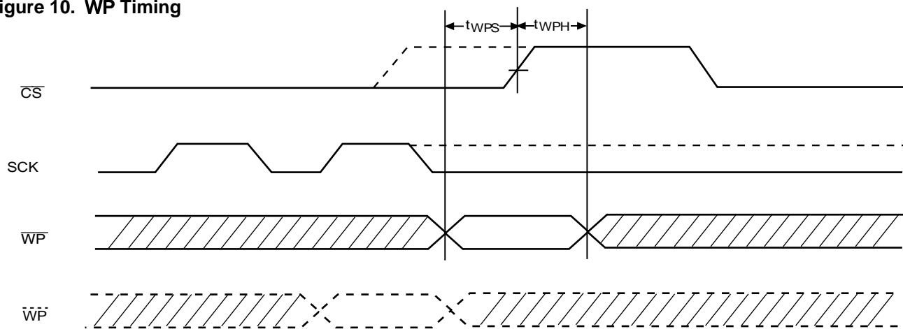
Figure 10. \overline{WP} Timing
