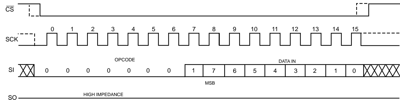
Figure 7. WRSR Timing
