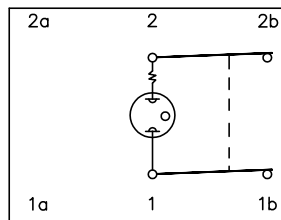
WIRING DIAGRAM SHOWING INTERNAL LAMP CONNECTIONS.
