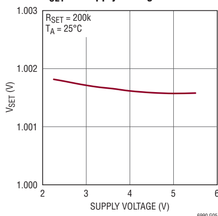
V_{\text{SET}} vs Supply Voltage
