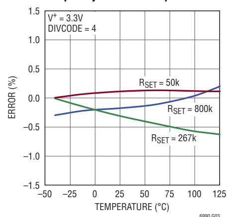
Frequency Error vs Temperature
