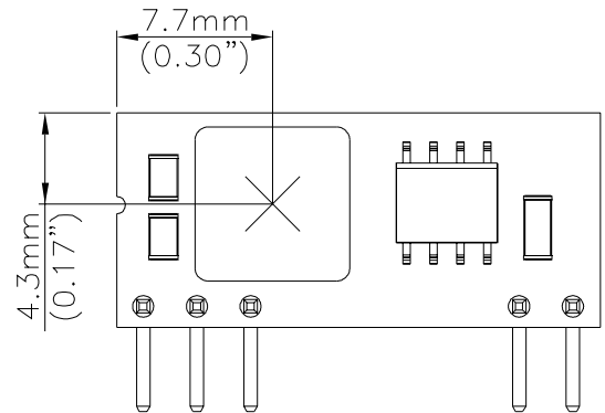
Figure 28: Temperature measurement location The allowed maximum hot spot temperature is defined at 125 .
