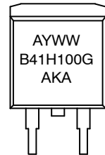
D 2 PAK CASE 418B STYLE 3
