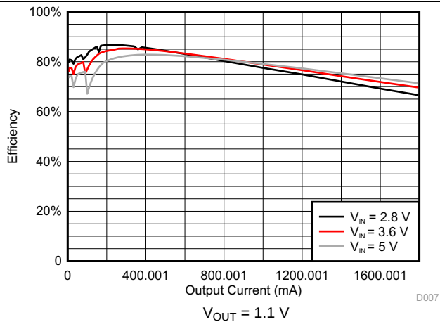
Figure 6-4. DCDC1/DCDC2 Efficiency
