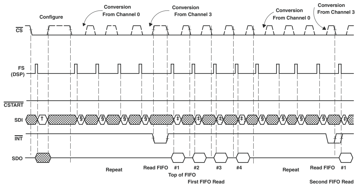
Figure 11. TLV2548 Mode 01 \mu\text{P}/\text{DSP} Serial Interface (Conversions Triggered by CSTART)
