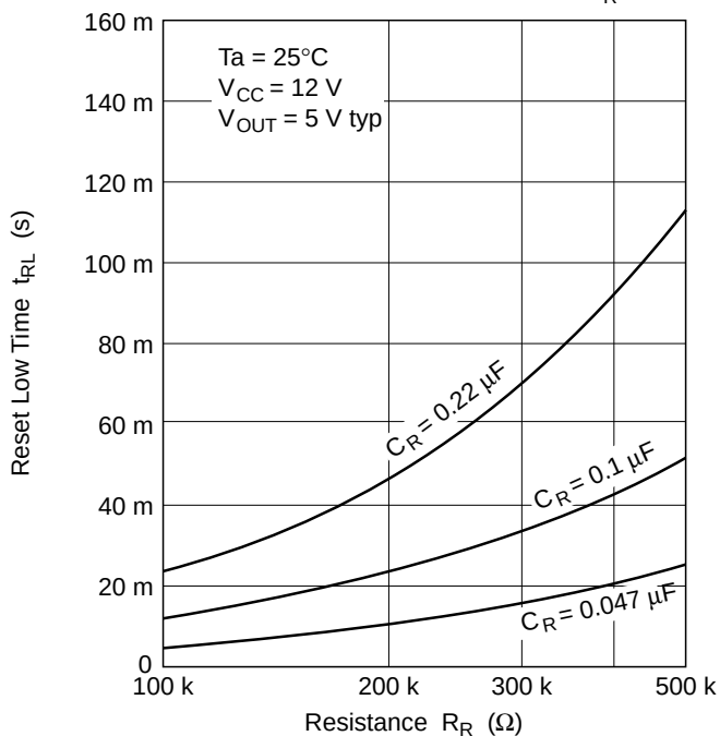
Reset Low Time vs. Resistance R_R
