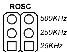
Figure 5. Watchdog-Oscillator Jumper
