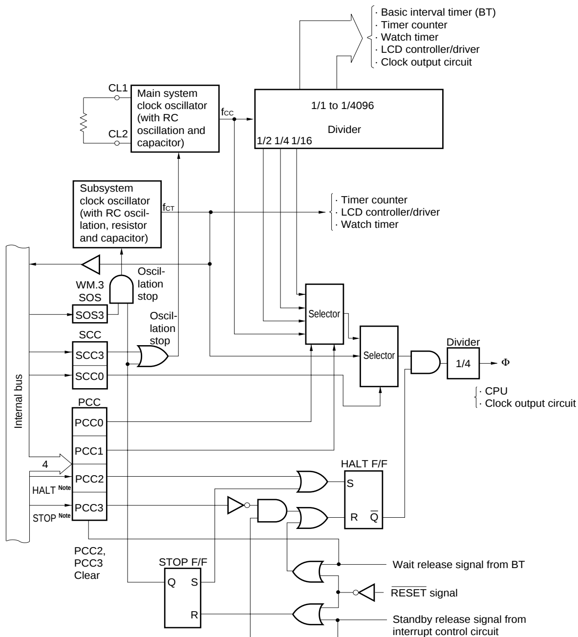
Figure 6-1. Clock Generator Block Diagram
