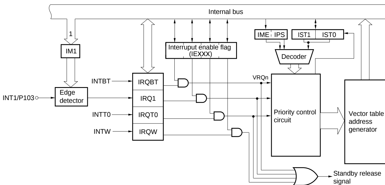
Figure 7-1. Interrupt Control Circuit Block Diagram
