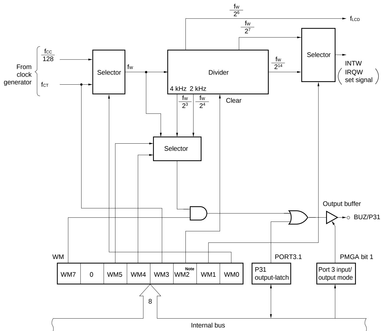
Figure 6-4. Watch Timer Block Diagram
