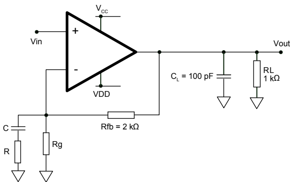
Figure 25. Low gain configuration
