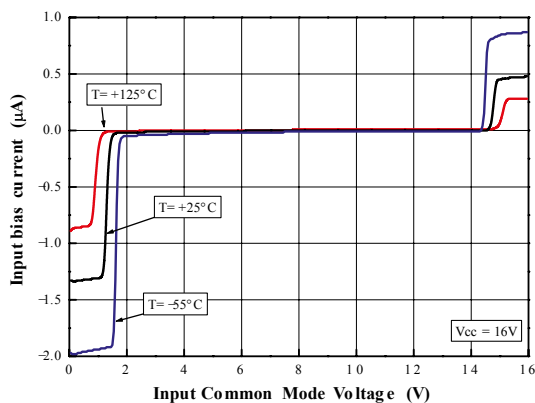
Figure 5. Input bias current vs. V_{icm} at V_{cc} = 16\text{V}
