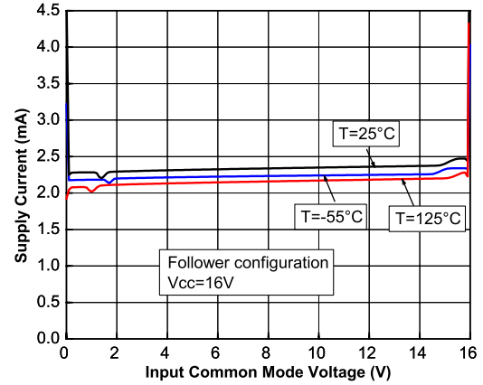
Figure 8. Supply current vs. V_{icm} in follower configuration at V_{CC} = 16\text{ V}
