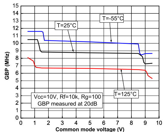
Figure 6. Gain bandwidth product vs. V_{icm} at V_{cc} = 10\text{V}
