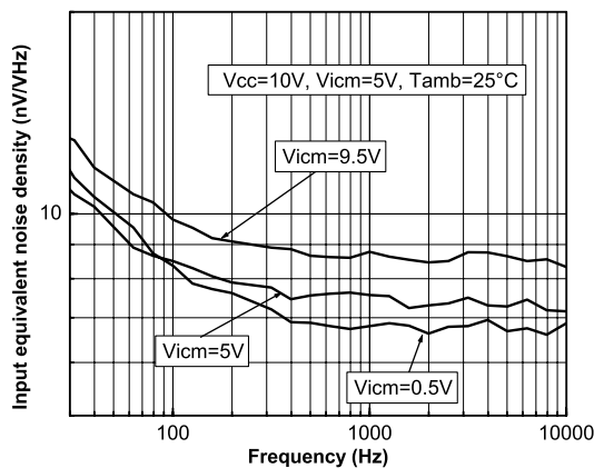
Figure 15. Noise vs. V_{icm} at V_{CC} = 10\text{ V}
