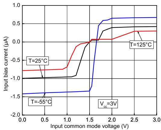
Figure 3. Input bias current vs. V_{icm} at V_{cc} = 3\text{V}
