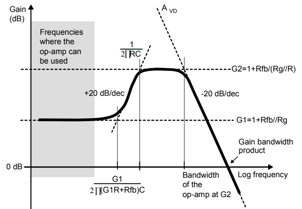
Figure 26. Closed-loop gain
