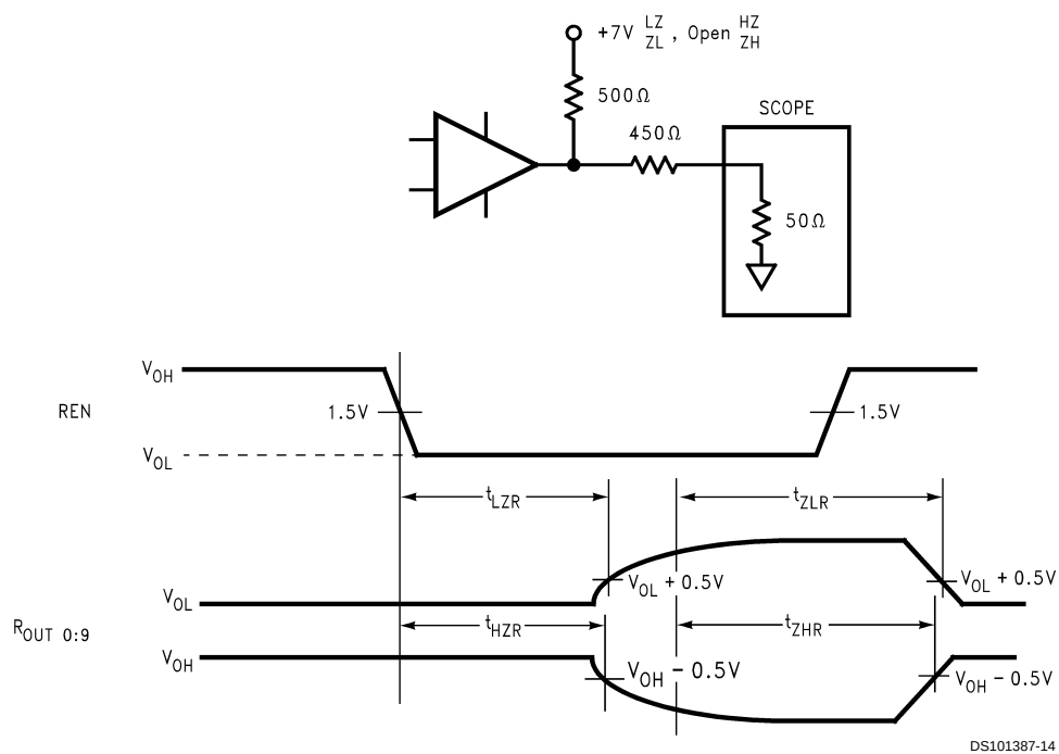
FIGURE 6. Deserializer TRI-STATE Test Circuit and Timing
