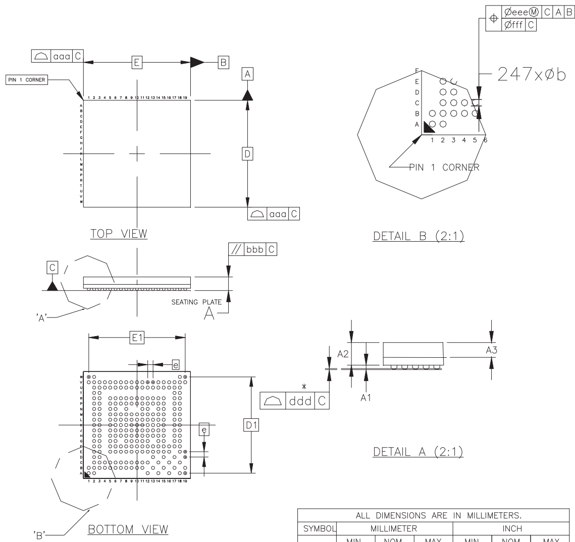
Figure 5-2. 247-ball BGA Package Drawing
