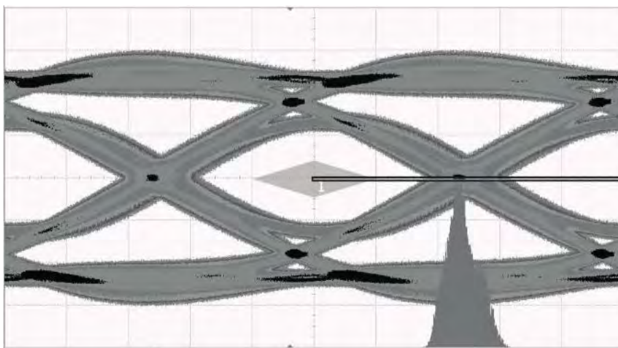
Fig 9. HDMI 2.0 TP2 eye diagram, PCB with PUSB3F97 (2160p, 60 Hz)
