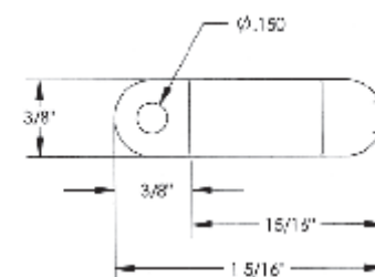
SPRING CLIP
