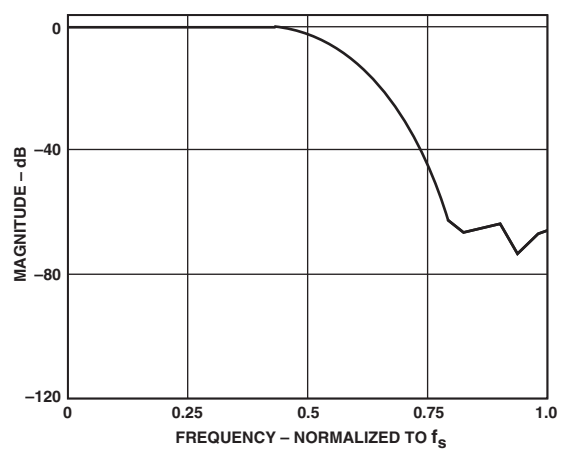
TPC 5. DAC Composite Filter Response Low Group Delay Enabled
