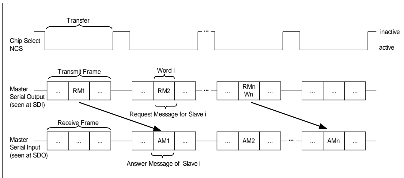
Figure 2-8 Response Answer Principle - Daisy Chain Topology
