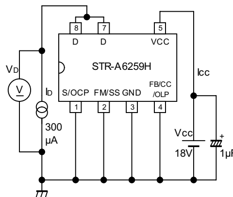
Measurement Circuit 7
