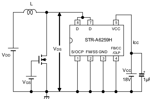
Measurement Circuit 7
