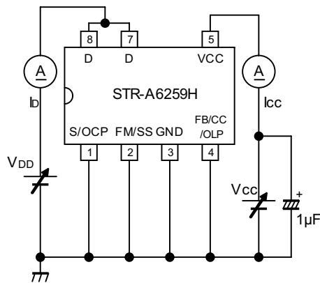
Measurement Circuit 5
