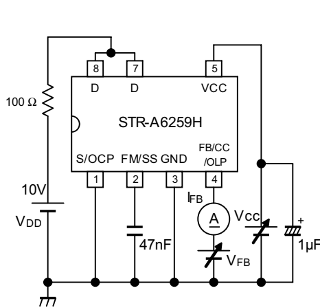
Measurement Circuit 5
