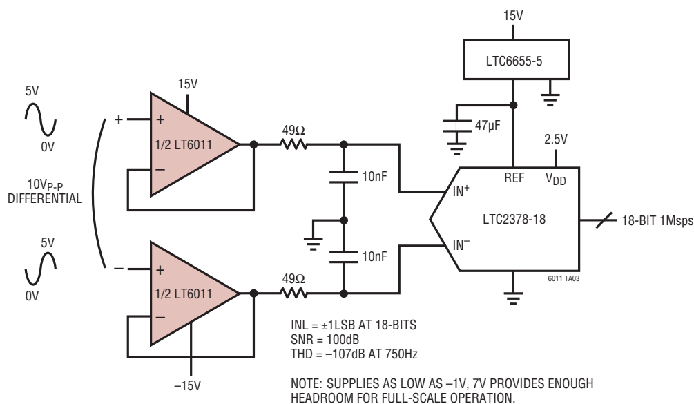
Buffering an 18-Bit 1Mps SAR ADC
