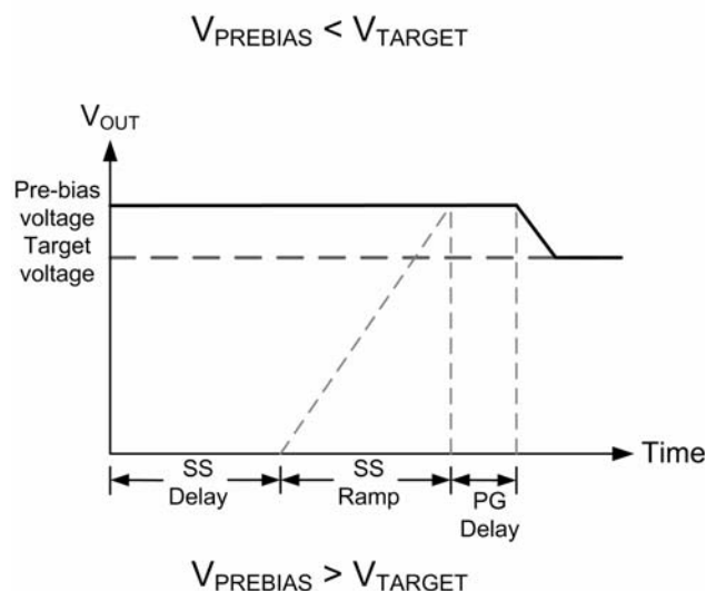
FIGURE 17. OUTPUT RESPONSES TO PRE-BIAS VOLTAGES
