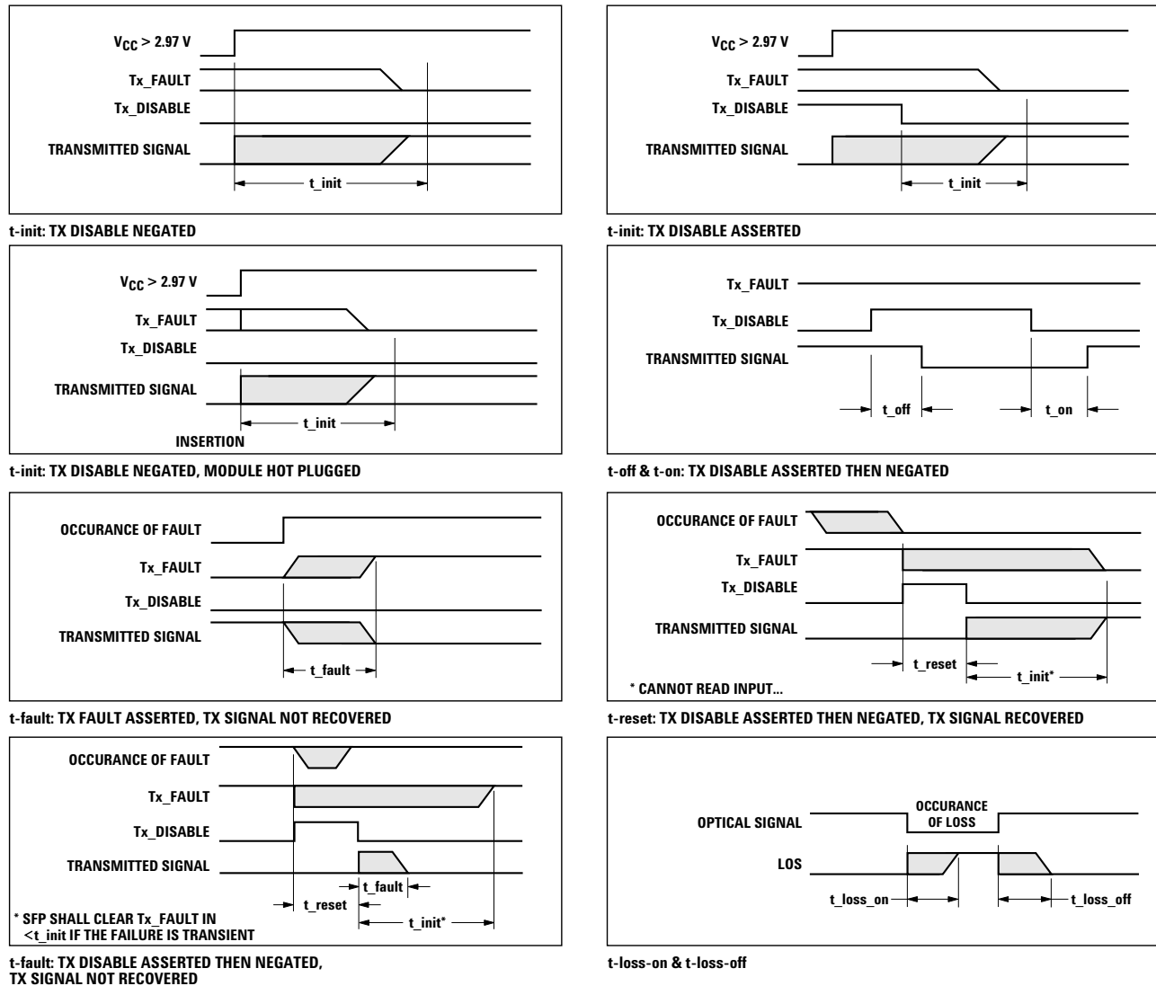
Figure 5. Transceiver Timing Diagrams (Module Installed Except Where Noted)
