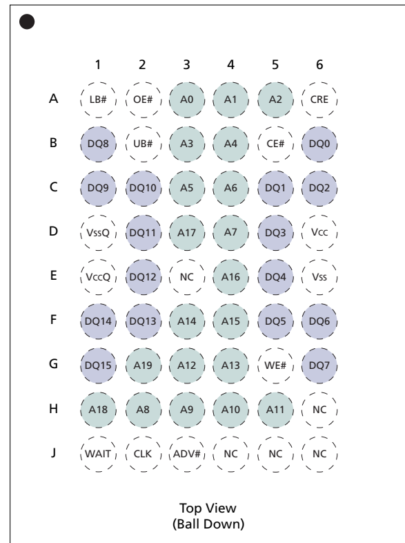
Figure 1: 54-Ball VFBGA
