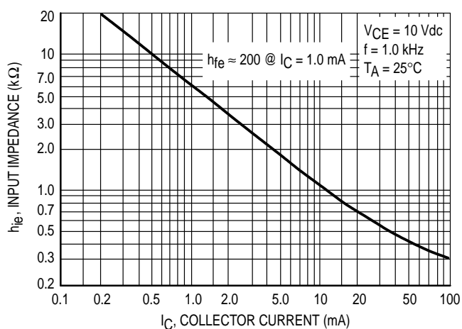
Figure 17. Input Impedance
