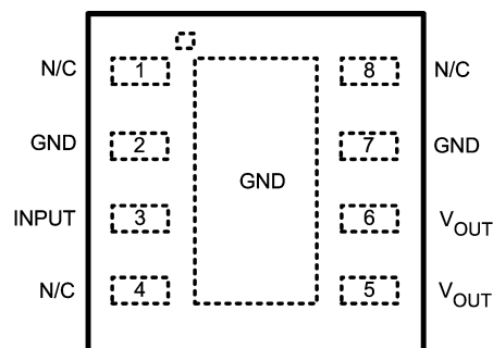
Top View Order Number LM2940LD-5.0, LM2940LD-8.0, LM2940LD-9.0, LM2940LD-10, LM2940LD-12, LM2940LD-15 See NS Package Number LDC08A
