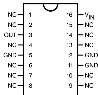
Top View See NS Package Number WG16A
