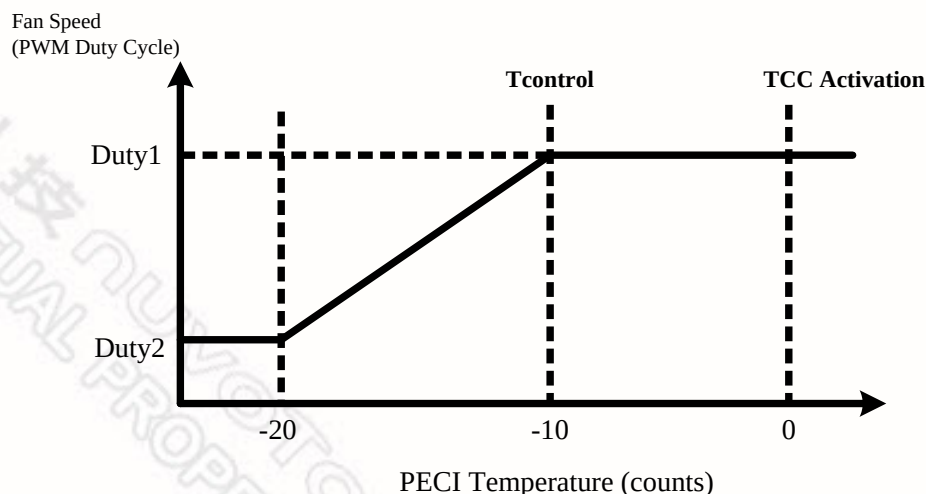
Figure 6-3 PECI Temperature
