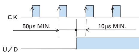
Pulse and direction mode ( CK, U/D )
