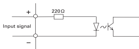
Input circuit configuration
