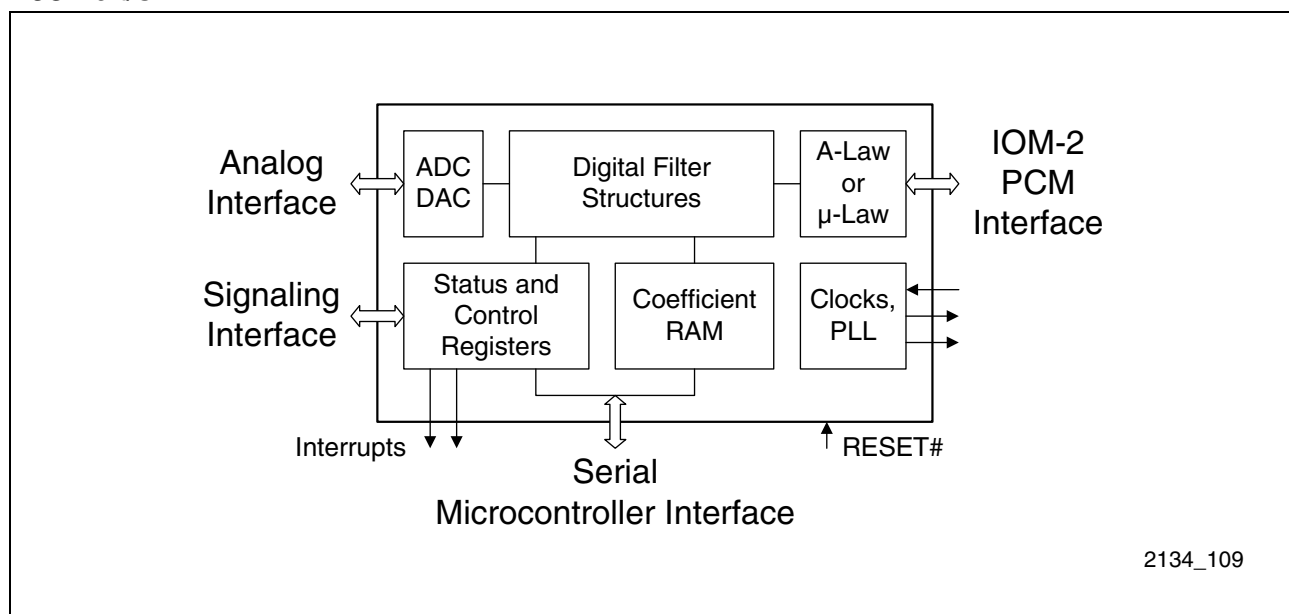
Figure 6 SICOFI®4-TE Interfaces
