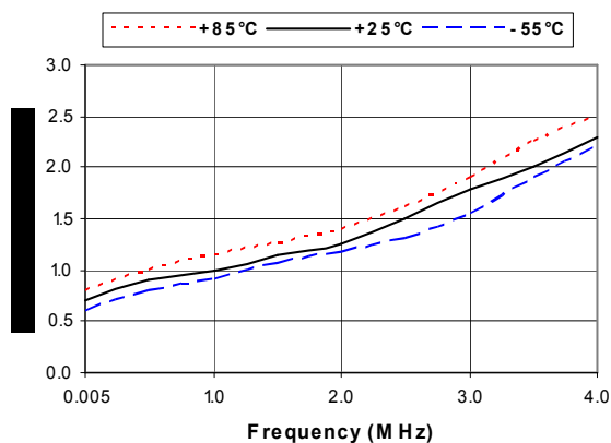
Insertion Loss
