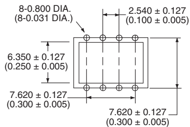
PCB Hole Pattern
