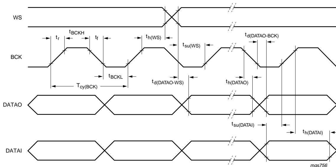
Fig 17. I 2 S-bus serial interface timing
