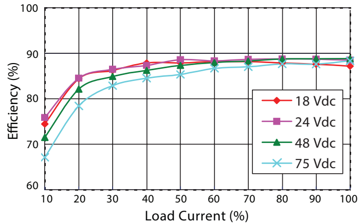
PDQ30-Q48-S3-D Efficiency Curve (Efficiency vs. Line Voltage and Load Current)
