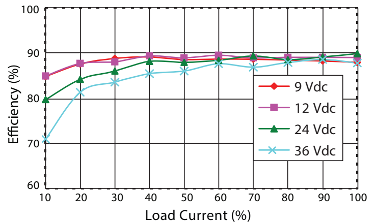
PDQ30-Q24-D12-D Efficiency Curve (Efficiency vs. Line Voltage and Load Current)
