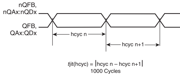
HALF-CYCLE JITTER
