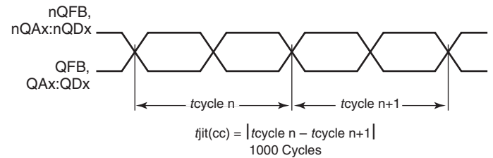
CYCLE-TO-CYCLE JITTER
