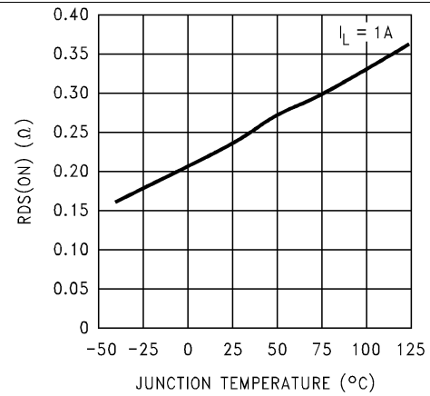
Figure 4. Drain-to-Source Resistance
