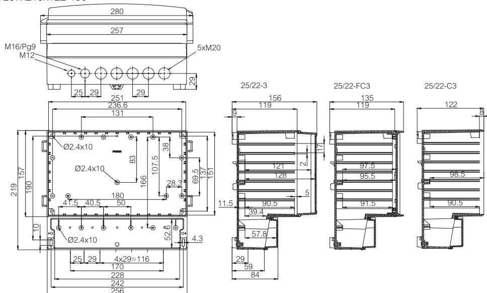
CARDMASTER 257x219x122-156
