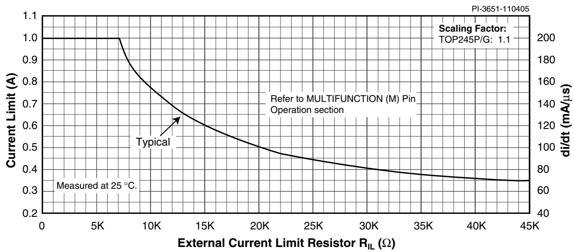
Figure 55b. Current Limit vs. External Current Limit Resistance (TOP245P/G only).
