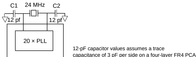
Figure 3-1. Crystal Configuration
