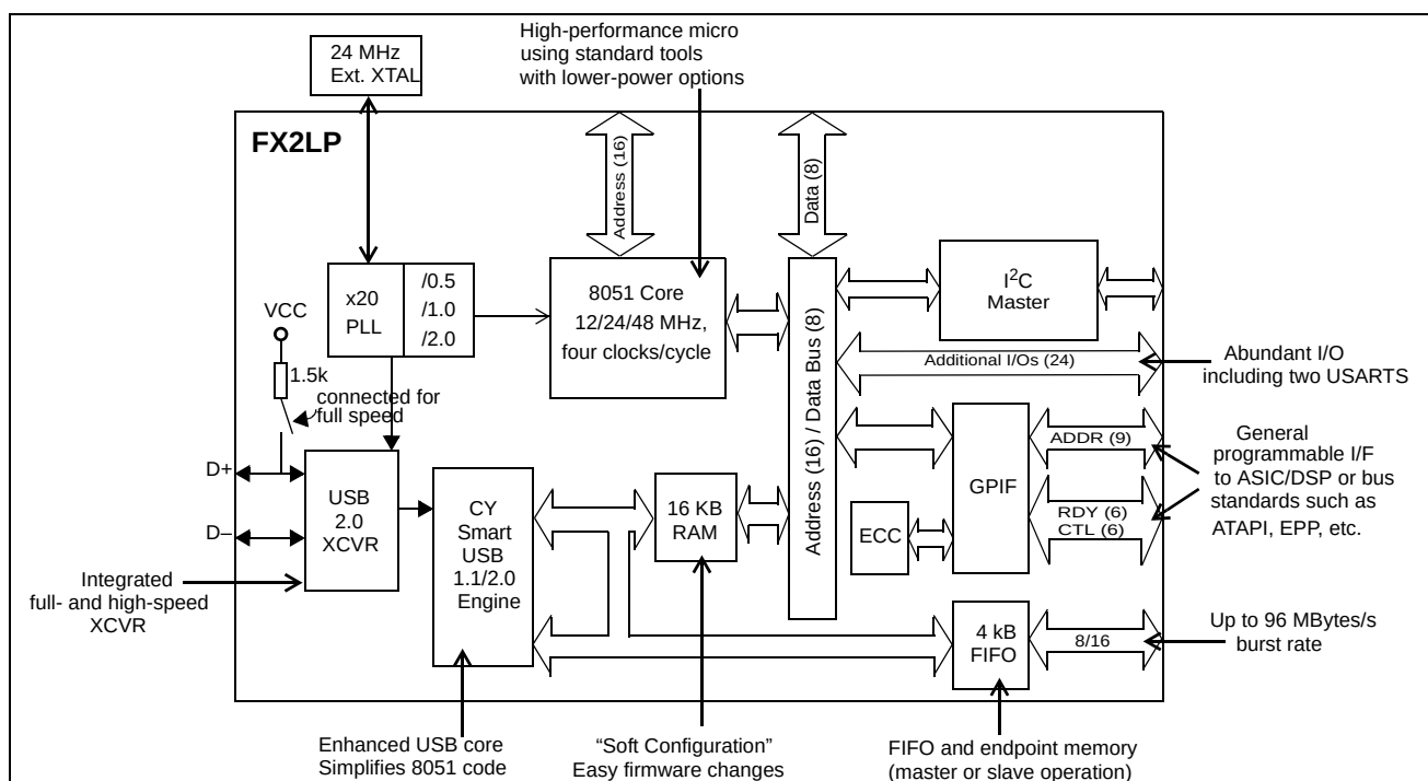
Figure 1-1. Block Diagram
