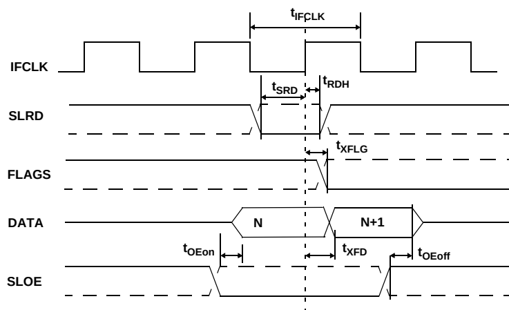
Figure 9-5. Slave FIFO Synchronous Read Timing Diagram [19]
