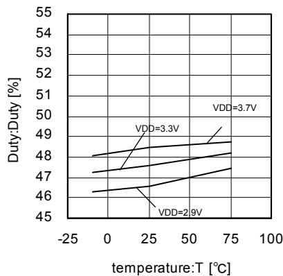
Fig.64 67.5MHz
