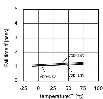
Fig.56 24.5454MHz Fall-time temperature characteristics
