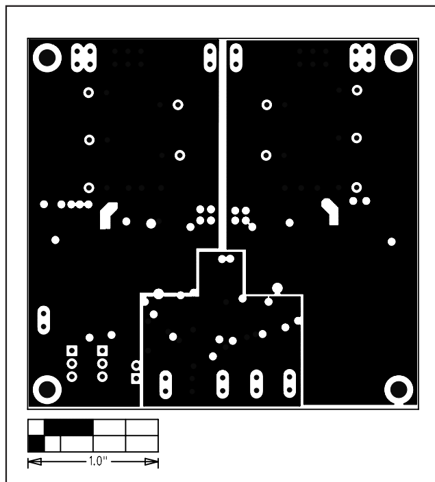
Figure 5. MAX8664 EV Kit PCB Layout—Inner Layer 2
