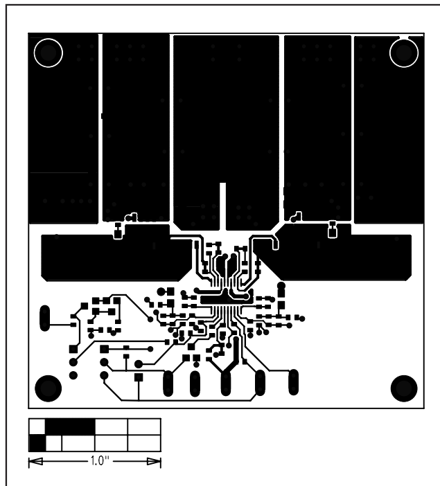
Figure 4. MAX8664 EV Kit PCB Layout—Component Side
