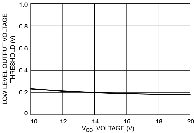
Figure 28. Low Level Output Voltage vs. Supply Voltage ( V_{CC} = V_{BOOT} )
