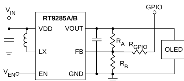
Figure 6. Application Circuit for Output Voltage Control and Related Equations
