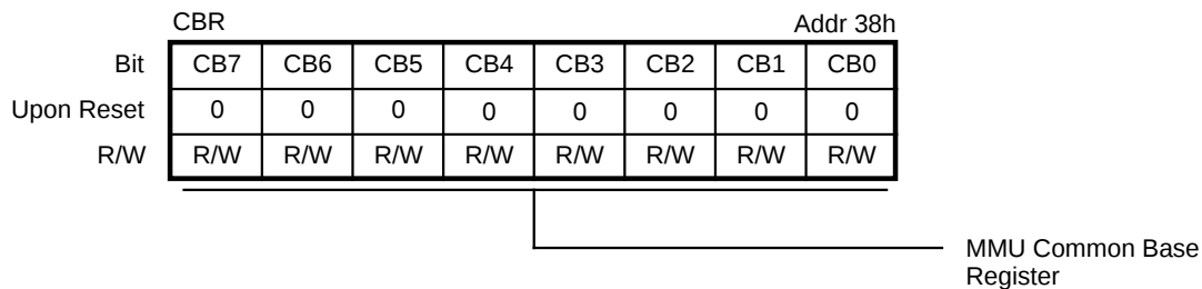
Figure 38. MMU Common Base Register
