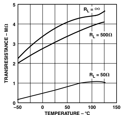
TPC 3. Transresistance vs. Temperature
