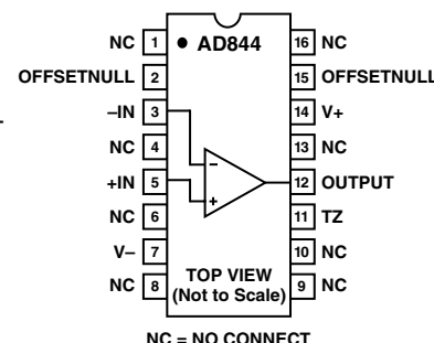
16-Lead SOIC (R) Package
