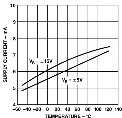
TPC 6. Quiescent Supply Current vs. Temperature and Supply Voltage
