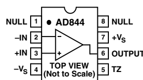
8-Lead Plastic (N), and Cerdip (Q) Packages
