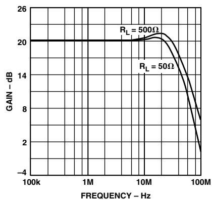
TPC 16. Gain vs. Frequency, Gain = -10
