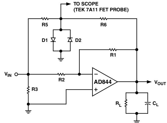
Figure 9. Settling Time Test Fixture
