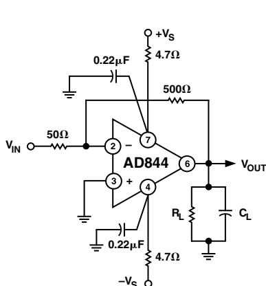
TPC 15. Gain of -10 Amplifier
