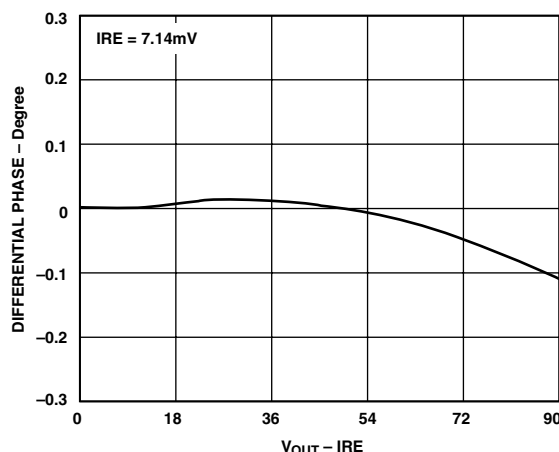
Figure 11c. Differential Phase for the Circuit of Figure 11a
