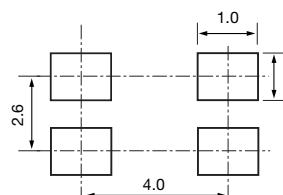
Figure 2) Land Pattern
