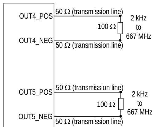
Figure 31. Recommended LVDS Output Port Line Termination
