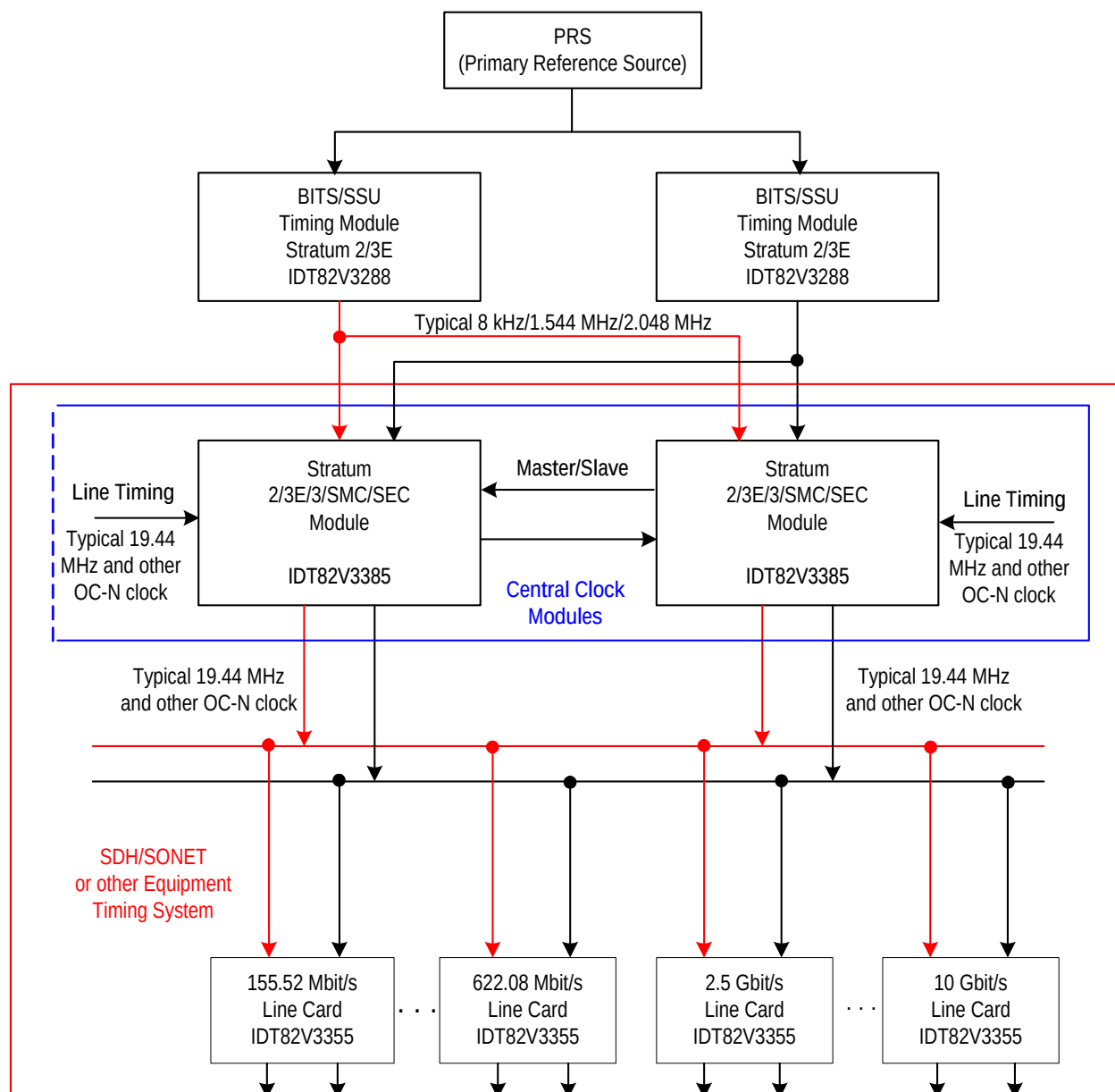
Figure 15. Typical Application
