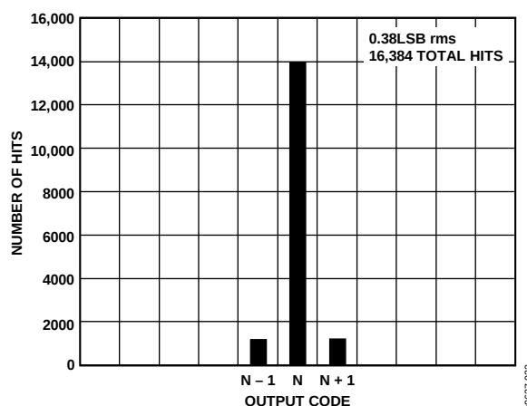
Figure 16. AD9613-170 Grounded Input Histogram
