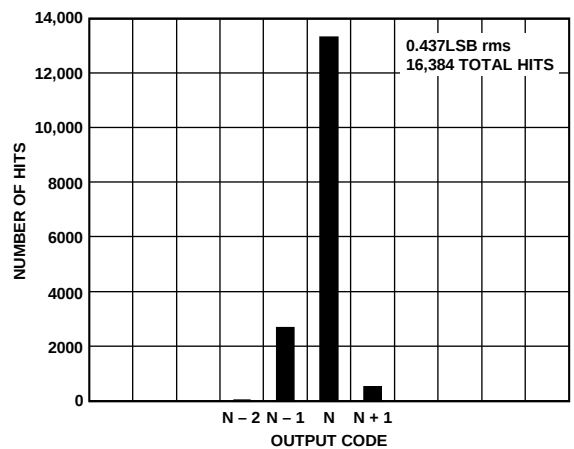
Figure 27. AD9613-210 Grounded Input Histogram
