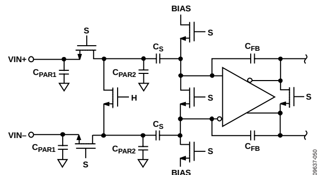
Figure 46. Switched-Capacitor Input
