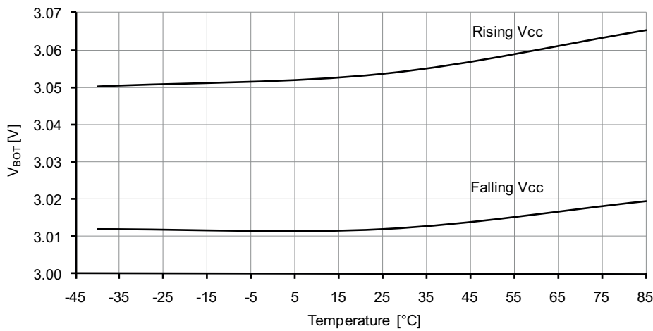
Figure 33-216. BOD thresholds vs. temperature. BOD level = 3.0V.
