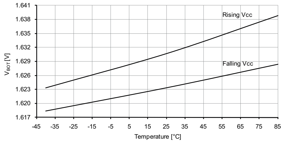
Figure 33-215. BOD thresholds vs. temperature. BOD level = 1.6V.
