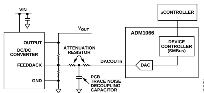
Figure 32. Open-Loop Margining System Using the ADM1066
