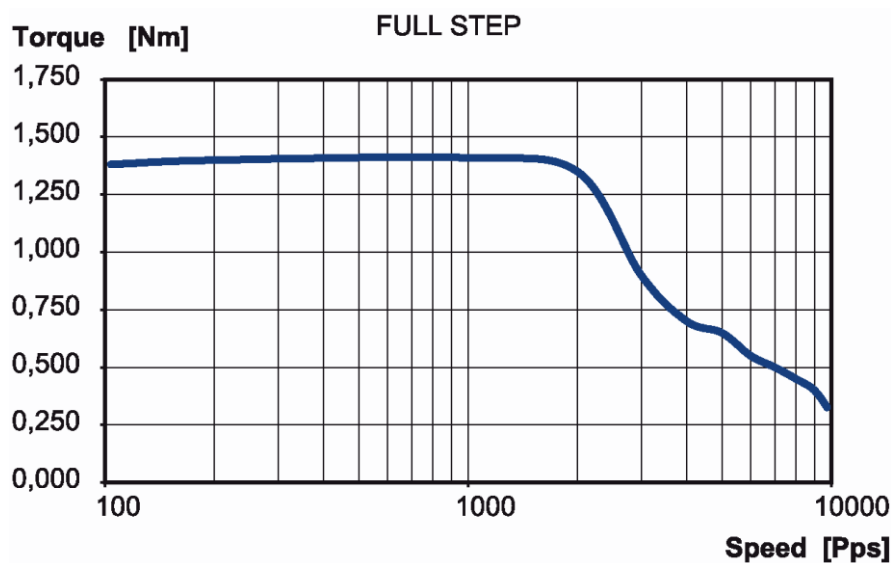
Figure 5.2: QSH6018-56-28-165 Speed vs. Torque Characteristics
