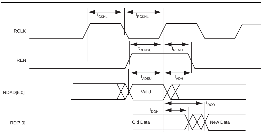
Figure 1-30 • 42MX SRAM Synchronous Read Operation
