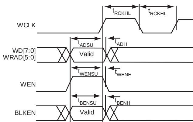
Figure 1-29 • 42MX SRAM Write Operation
