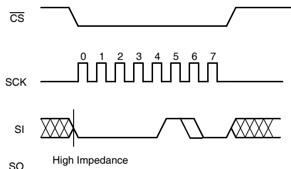
FIGURE 5. WRITE ENABLE/DISABLE LATCH SEQUENCE (WREN/WRDI INSTRUCTION)
